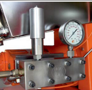
Stainless steel pump-head
